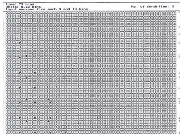
Fig. 5. The results of the TCNN simulation with input firings each 9 and 13 bins (i.e. two coded stimuli of different frequencies corresponding to the interspike intervals 9 and 13 bins). The network parameters are in the top window. The window below contains a TCNN spatio-temporal plane (PE arranged according to 'tuned' frequency on the abscissa, time on ordinate; the PE tuned to 1 bin interspike interval in time 0 at the upper left corner). 'I' symbols in the right-hand column indicate appearance of discharges on input to the network at the given moment. Discharging PE are marked as black circles. Discharges are distributed in time among the 9th, 18th, 27th, 36th and 13th, 26th processing elements, thus indicating a transformation to place code. For non-stationary short tone stimuli the frequency resolution of this mechanism is supposed to exceed the range of place code resolution. The transformation of temporal code to place code is in agreement with physiological observations. It further enables an information interchange between the place code and the temporal code (originating in the cochlea) in the higher stages of auditory processing
