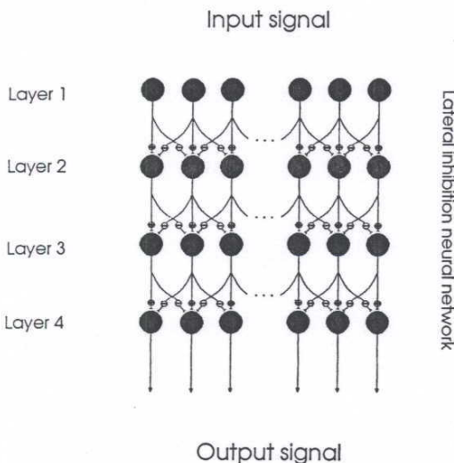
Fig. 1. The architecture of a lateral inhibition neural network (LINN)
