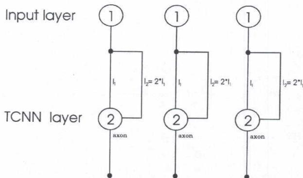
Fig. 3. The temporal coincidence neural network (TCNN). Note the different lengths of (dendrites) which constitute the frequency filter. Thresholds of the TCNN processing elements (PEs) are twice as high as those in the input layer. PEs are arranged according to their l_1 value
